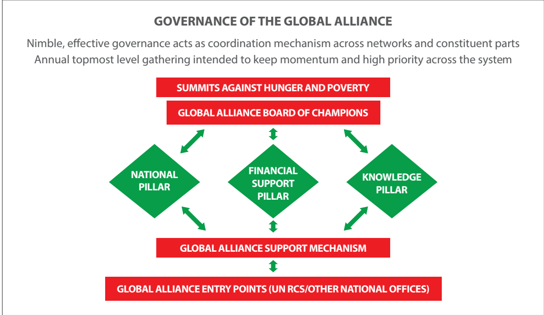
FIGURE 5. Governance mechanisms
